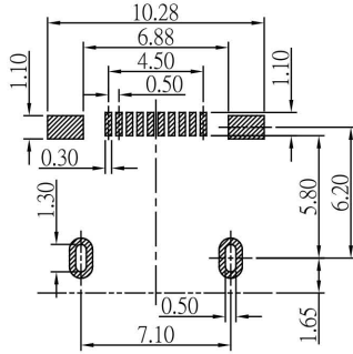
Recommended PCB Layout (PCB TOLERANCE \pm 0.05 )
