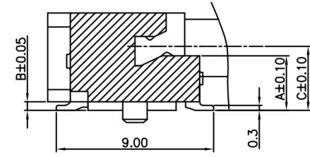
B-B' SECTION
