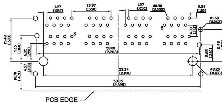
SUGGESTED PCB LAYOUT TOP VIEW
